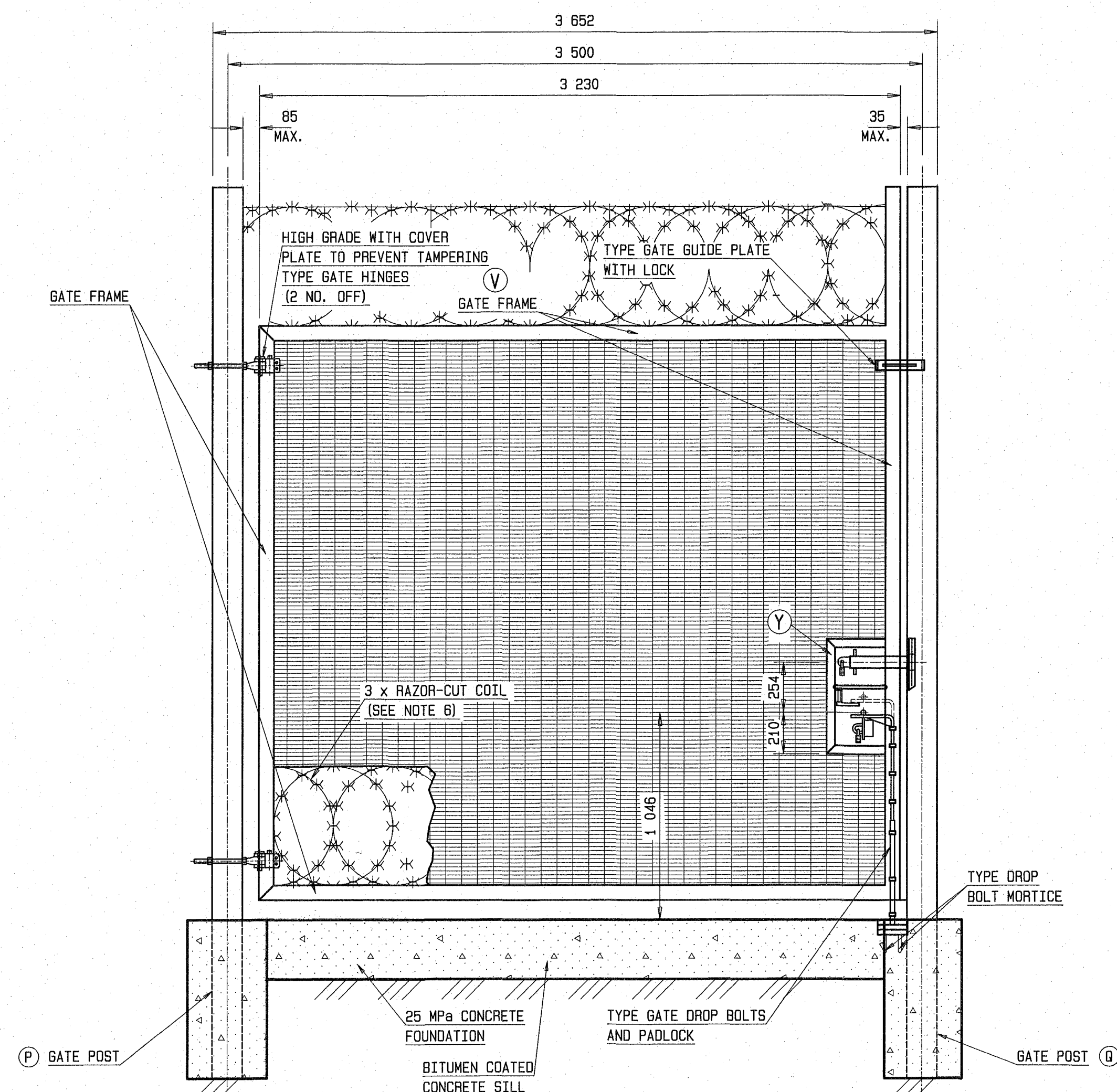
INSIDE ELEVATION OF BOUNDARY GATE
